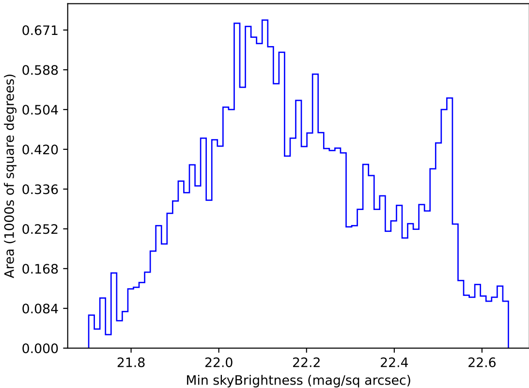
roman_v3.3_10yrs All sky u band: Min skyBrightness
