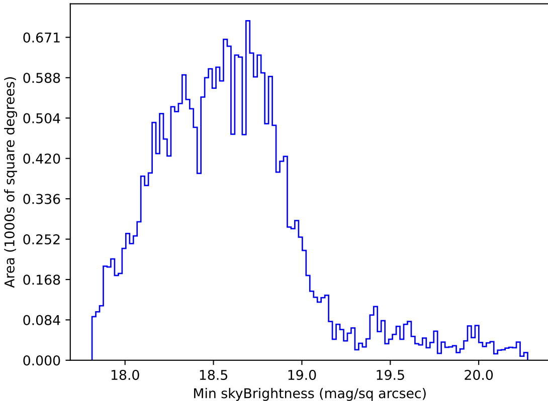
roman_v3.3_10yrs All sky r band: Min skyBrightness
