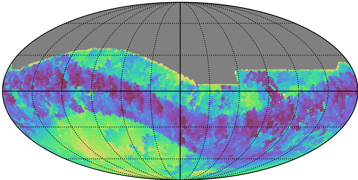
roman_v3.3_10yrs All sky i band: Min skyBrightness
