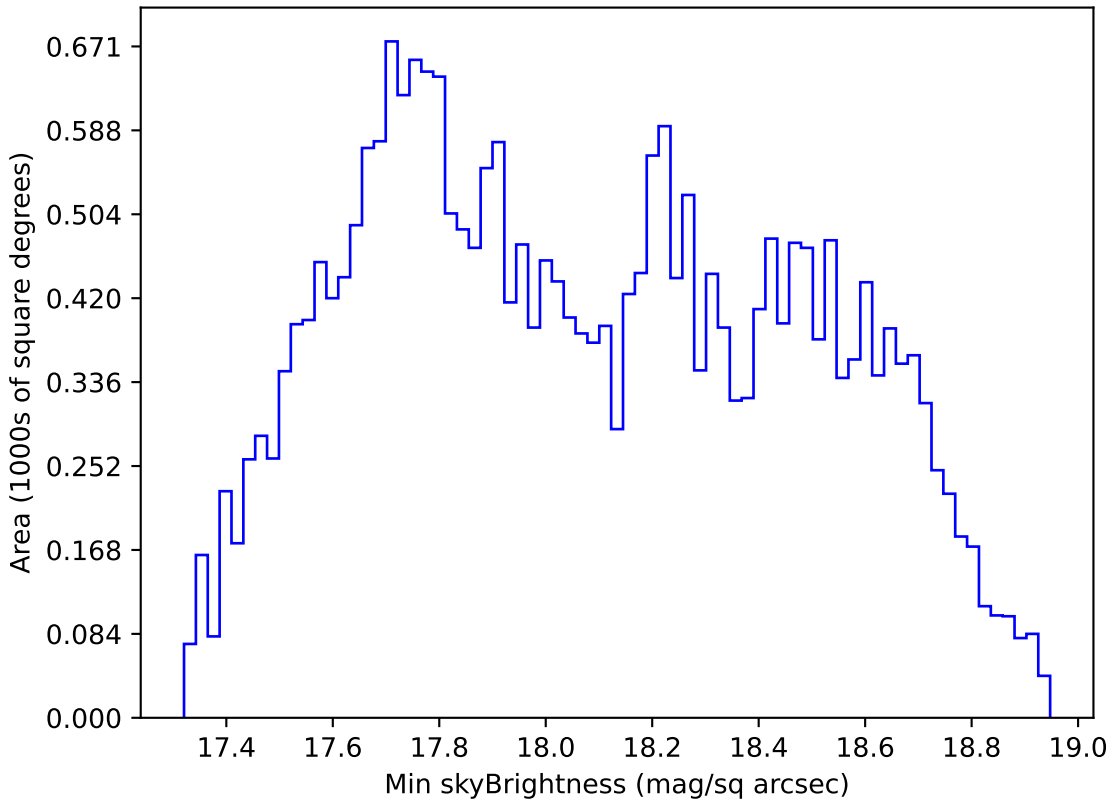
roman_v3.3_10yrs All sky i band: Min skyBrightness
