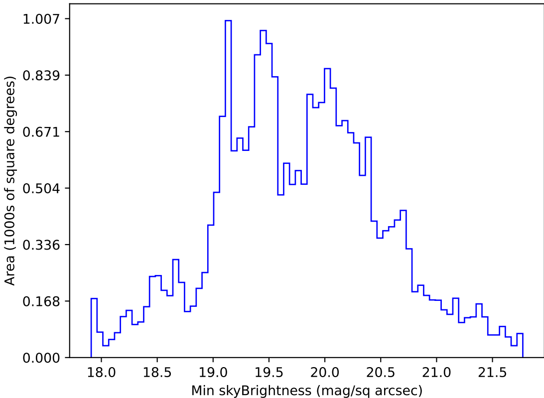
roman_v3.3_10yrs All sky g band: Min skyBrightness
