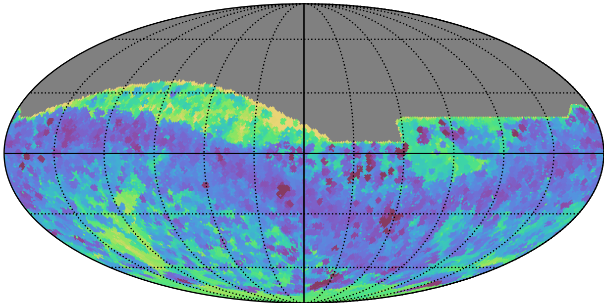
roman_v3.3_10yrs All sky all bands: Min skyBrightness
