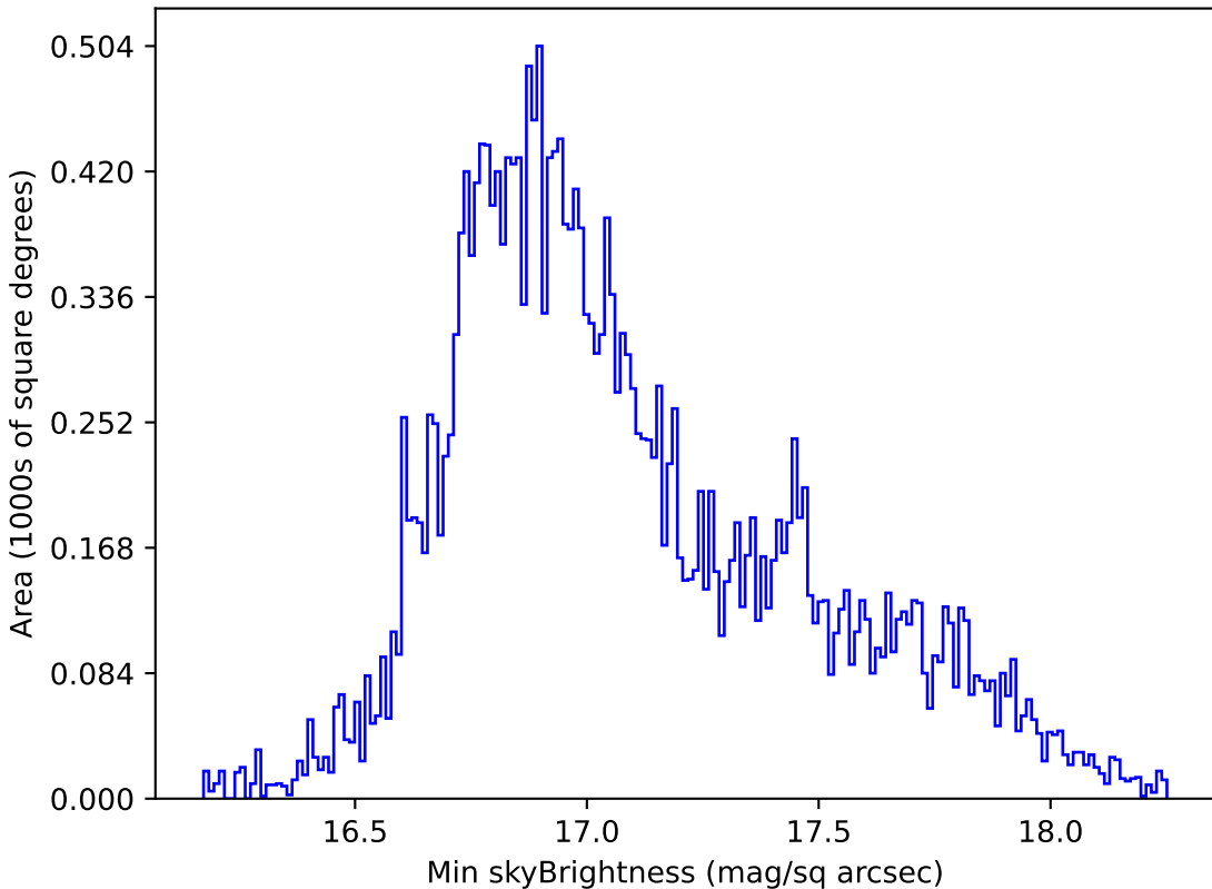
roman_v3.3_10yrs All sky all bands: Min skyBrightness
