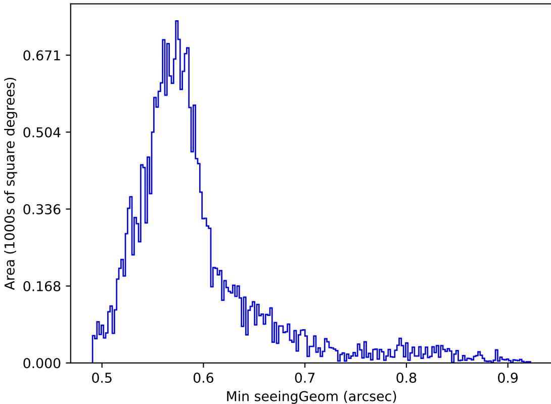
roman_v3.3_10yrs Yr 1 all bands: Min seeingGeom
