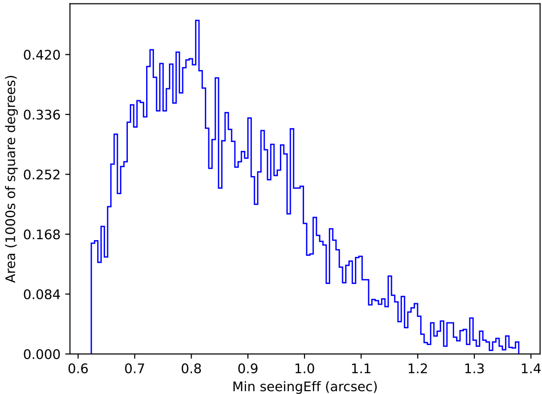
roman_v3.3_10yrs Yr 1 u band: Min seeingEff
