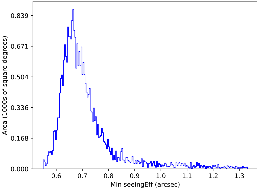
roman_v3.3_10yrs Yr 1 r band: Min seeingEff
