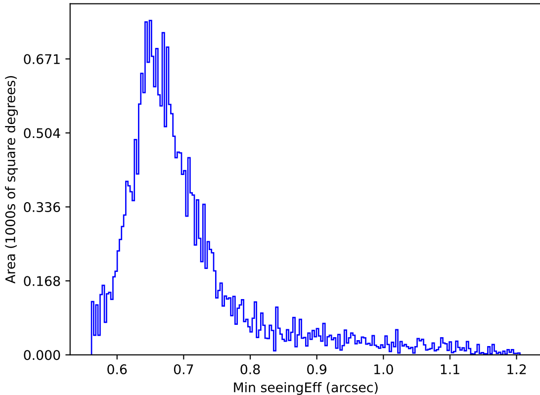
roman_v3.3_10yrs Yr 1 i band: Min seeingEff
