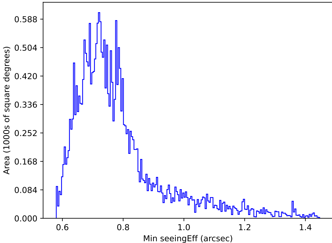
roman_v3.3_10yrs Yr 1 g band: Min seeingEff
