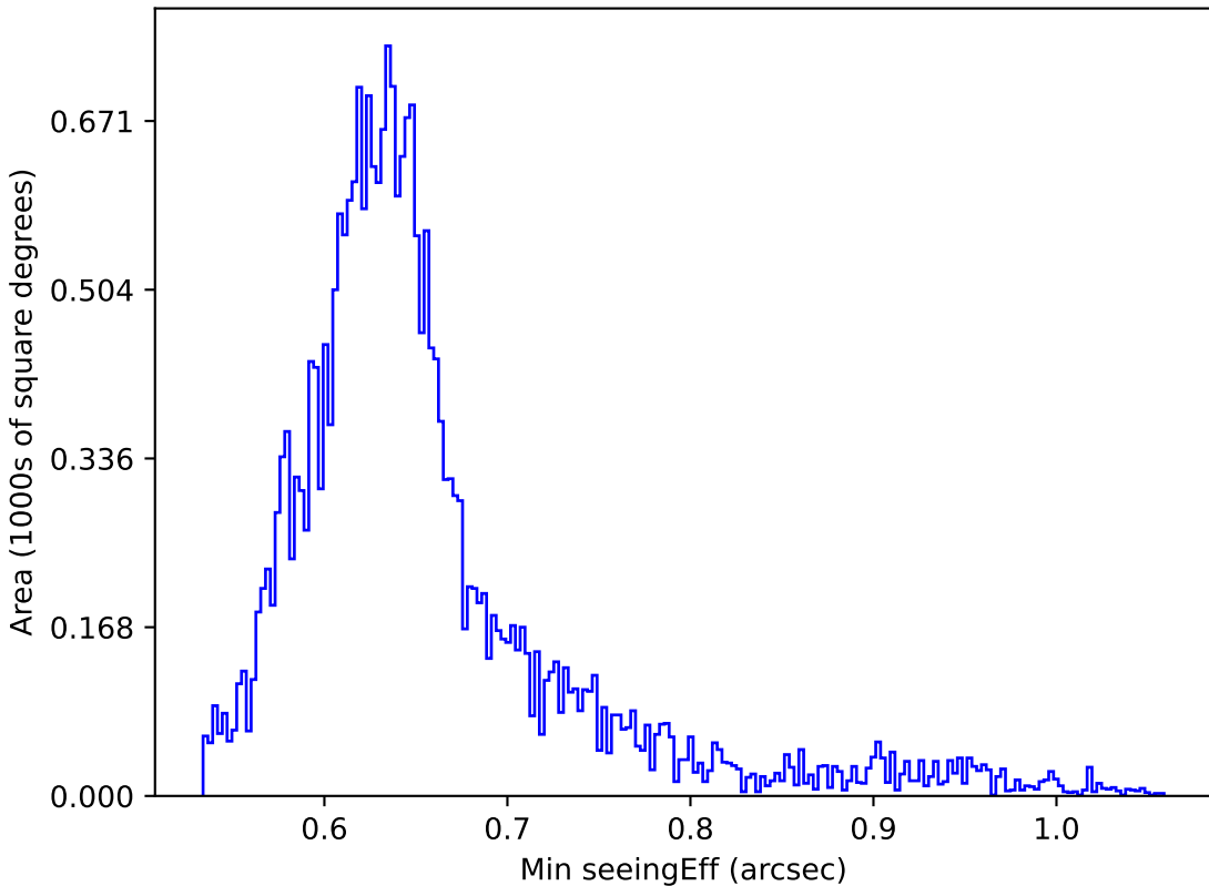
roman_v3.3_10yrs Yr 1 all bands: Min seeingEff
