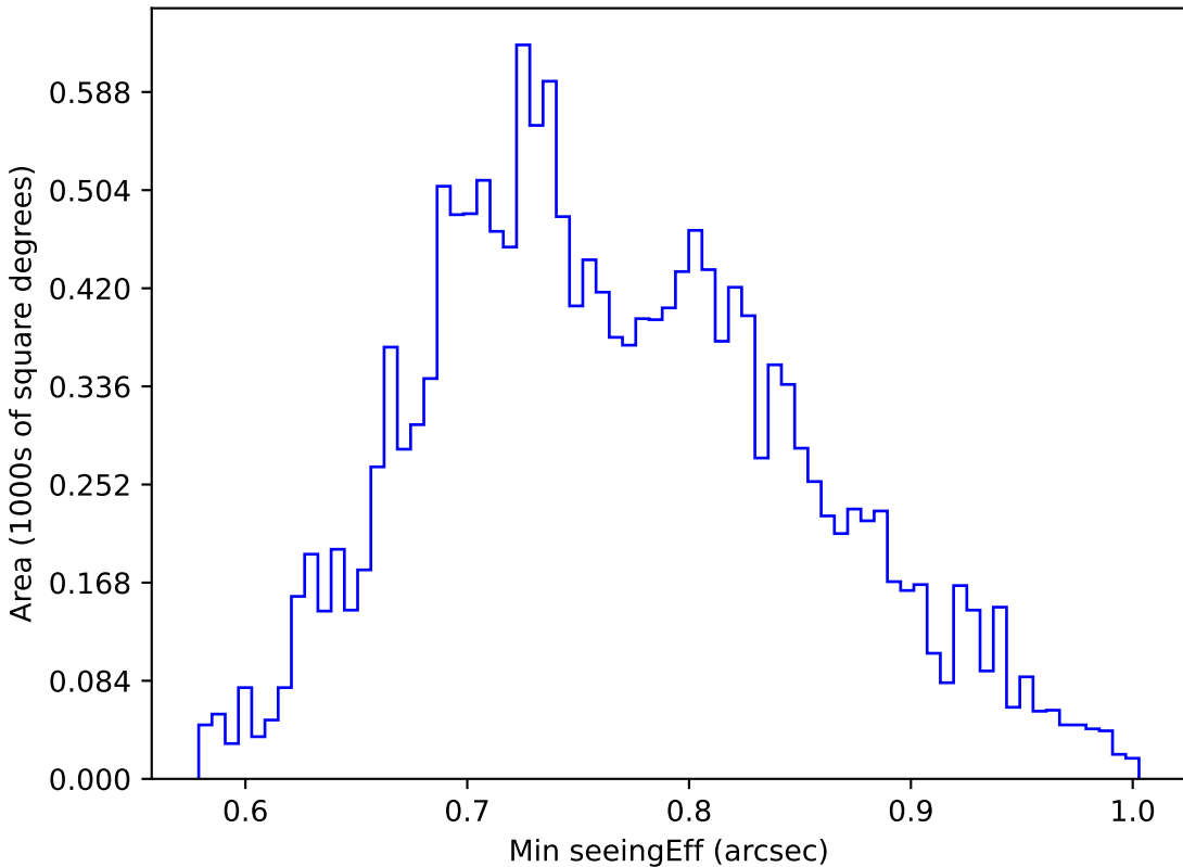
roman_v3.3_10yrs WFD u band: Min seeingEff
