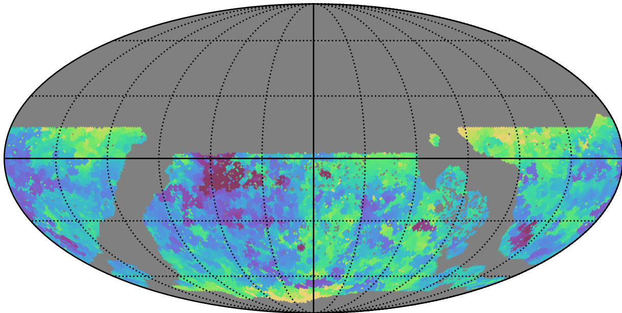
roman_v3.3_10yrs WFD g band: Min seeingEff
