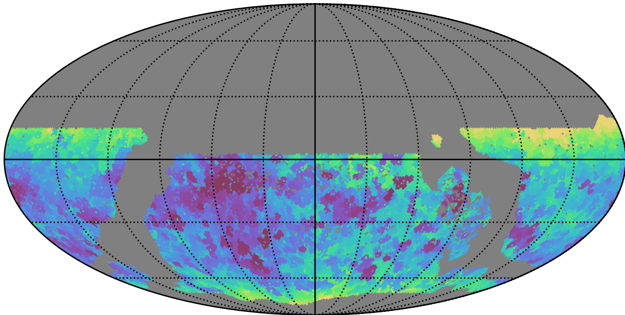
roman_v3.3_10yrs WFD all bands: Min seeingEff
