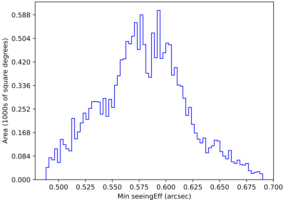
roman_v3.3_10yrs WFD all bands: Min seeingEff
