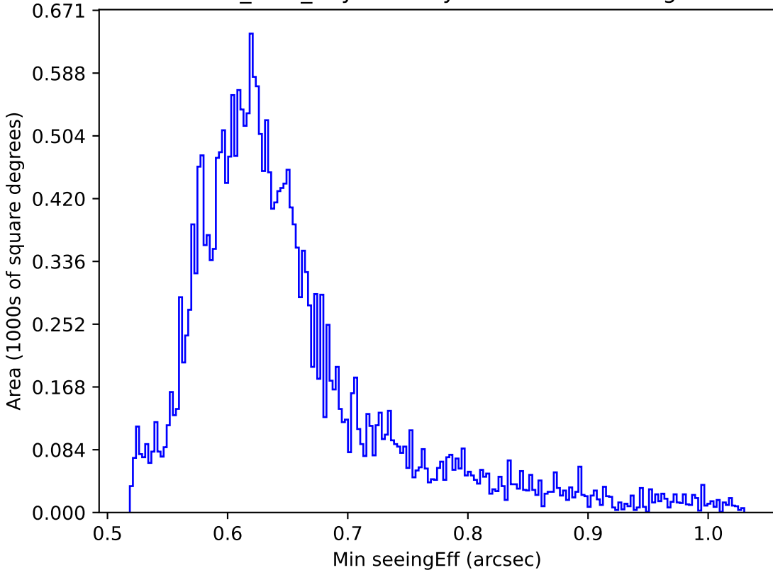
roman_v3.3_10yrs All sky z band: Min seeingEff
