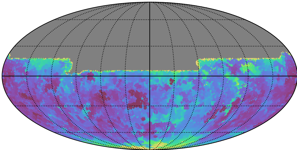
roman_v3.3_10yrs All sky u band: Min seeingEff
