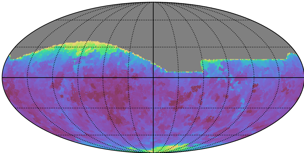
roman_v3.3_10yrs All sky r band: Min seeingEff
