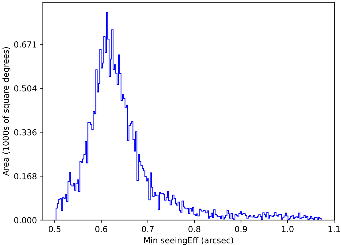
roman_v3.3_10yrs All sky r band: Min seeingEff
