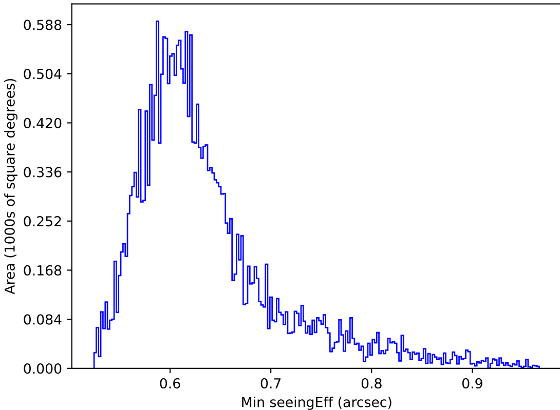
roman_v3.3_10yrs All sky i band: Min seeingEff
