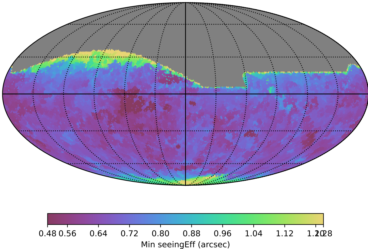
roman_v3.3_10yrs All sky g band: Min seeingEff
