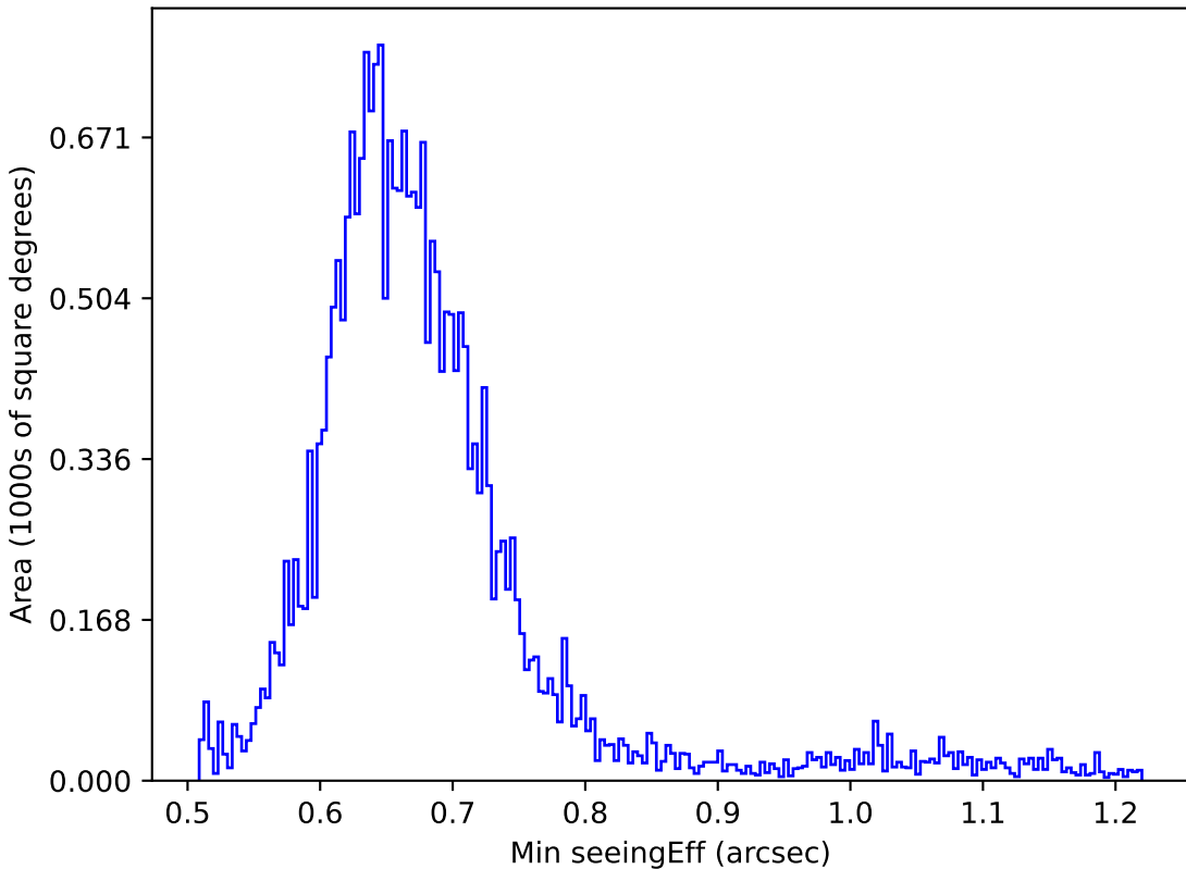
roman_v3.3_10yrs All sky g band: Min seeingEff
