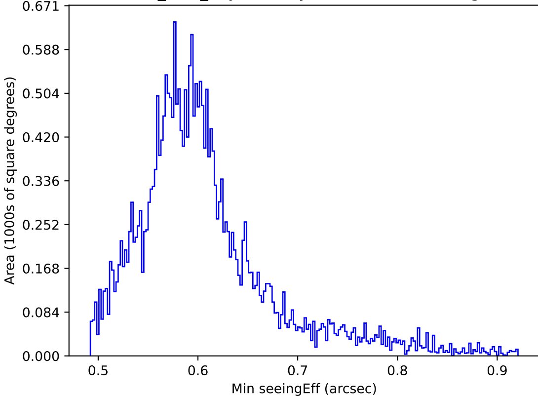
roman_v3.3_10yrs All sky all bands: Min seeingEff
