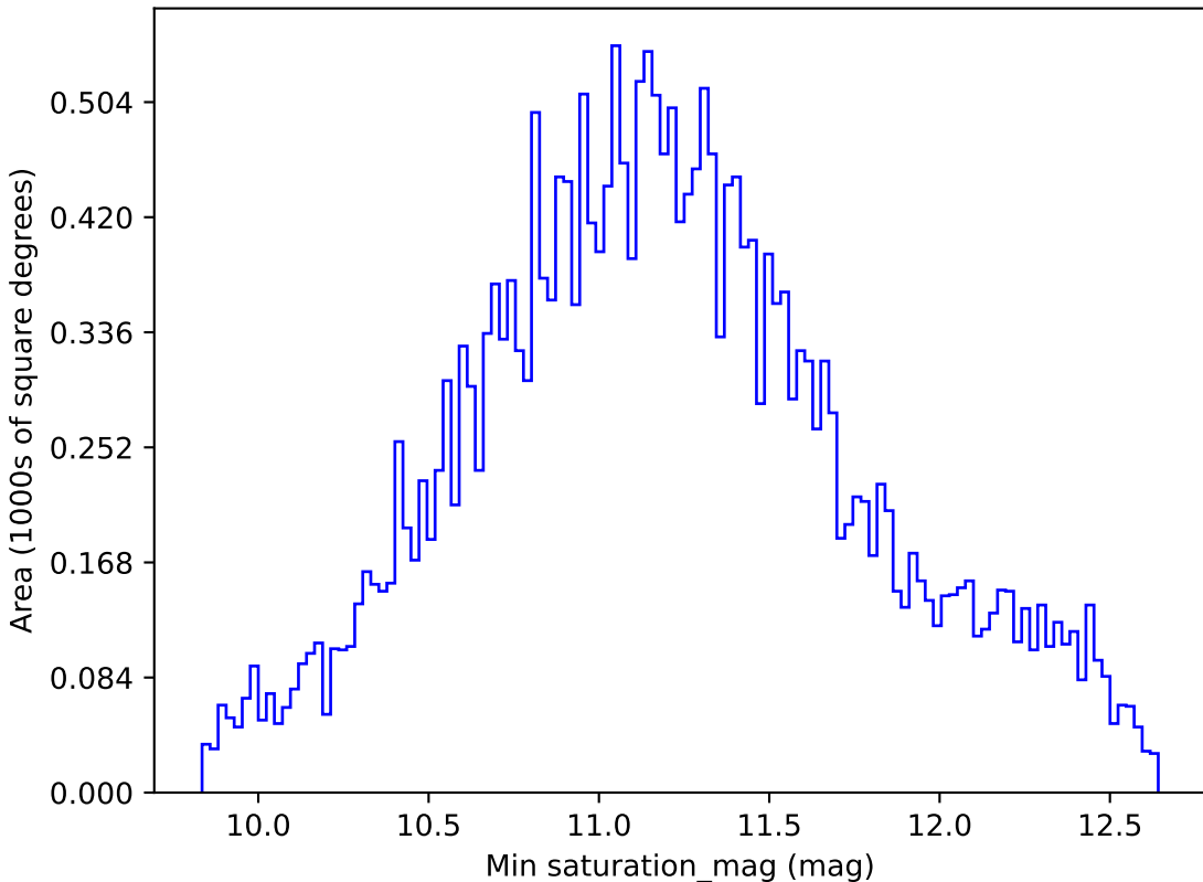
roman_v3.3_10yrs All sky all bands: Min saturation_mag
