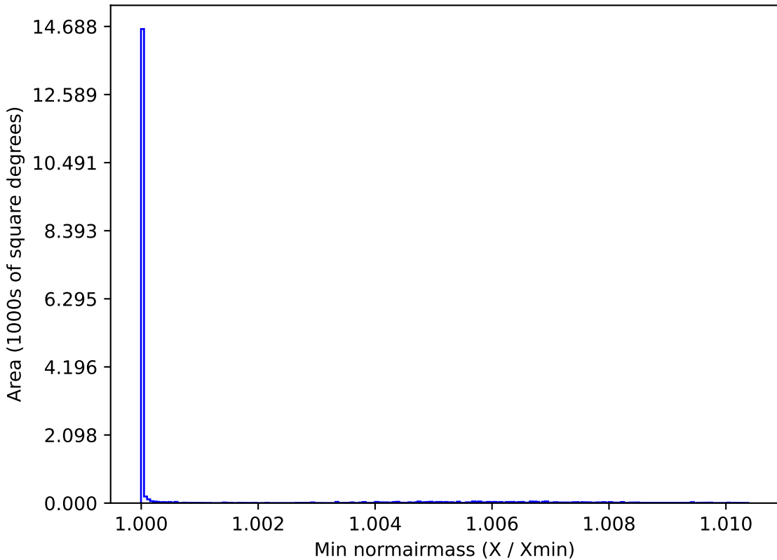
roman_v3.3_10yrs WFD all bands: Min normairmass
