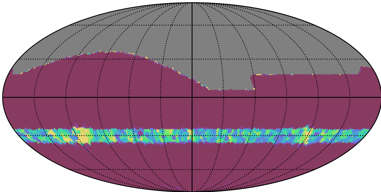
roman_v3.3_10yrs All sky all bands: Min normairmass
