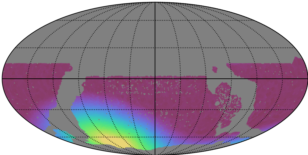
roman_v3.3_10yrs WFD all bands: Min moonDistance
