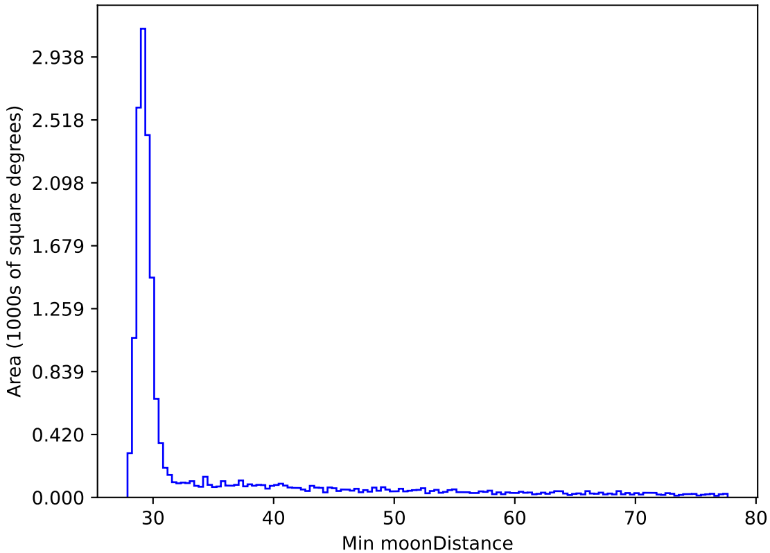
roman_v3.3_10yrs WFD all bands: Min moonDistance
