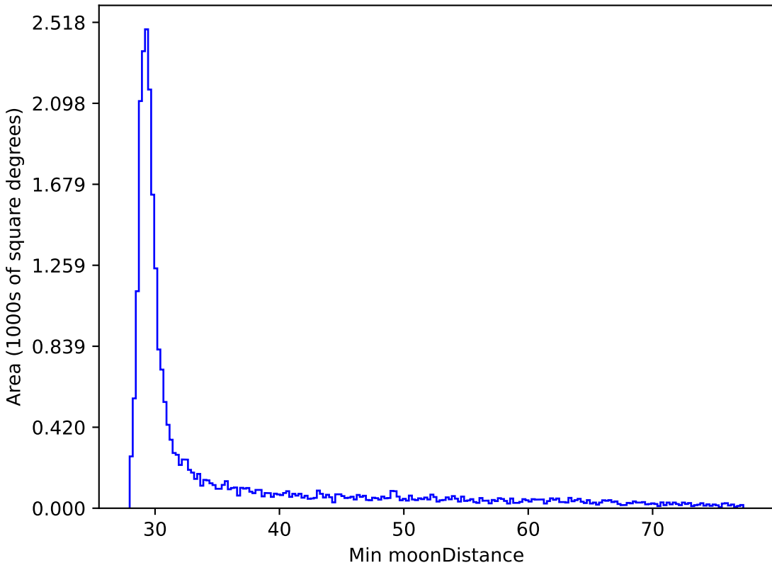
roman_v3.3_10yrs All sky all bands: Min moonDistance
