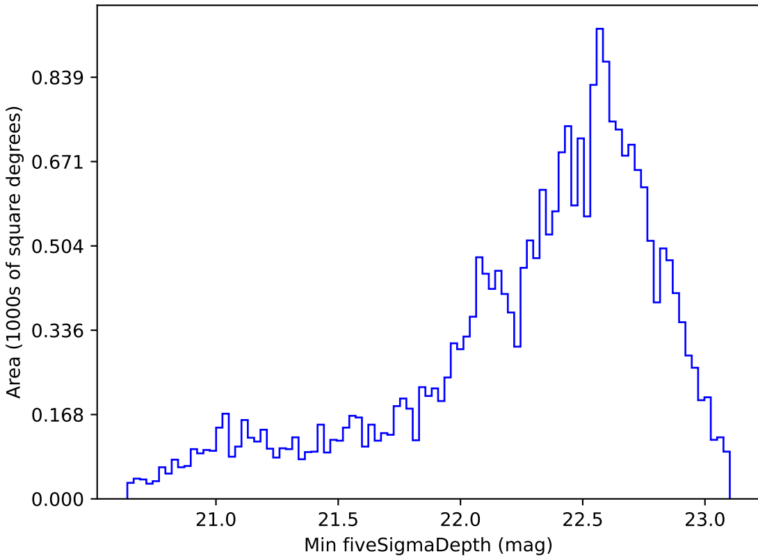
roman_v3.3_10yrs Yr 1 z band: Min fiveSigmaDepth
