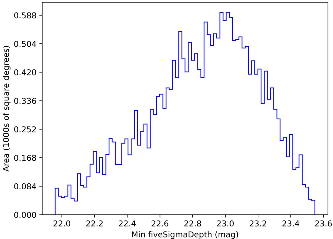
roman_v3.3_10yrs Yr 1 u band: Min fiveSigmaDepth
