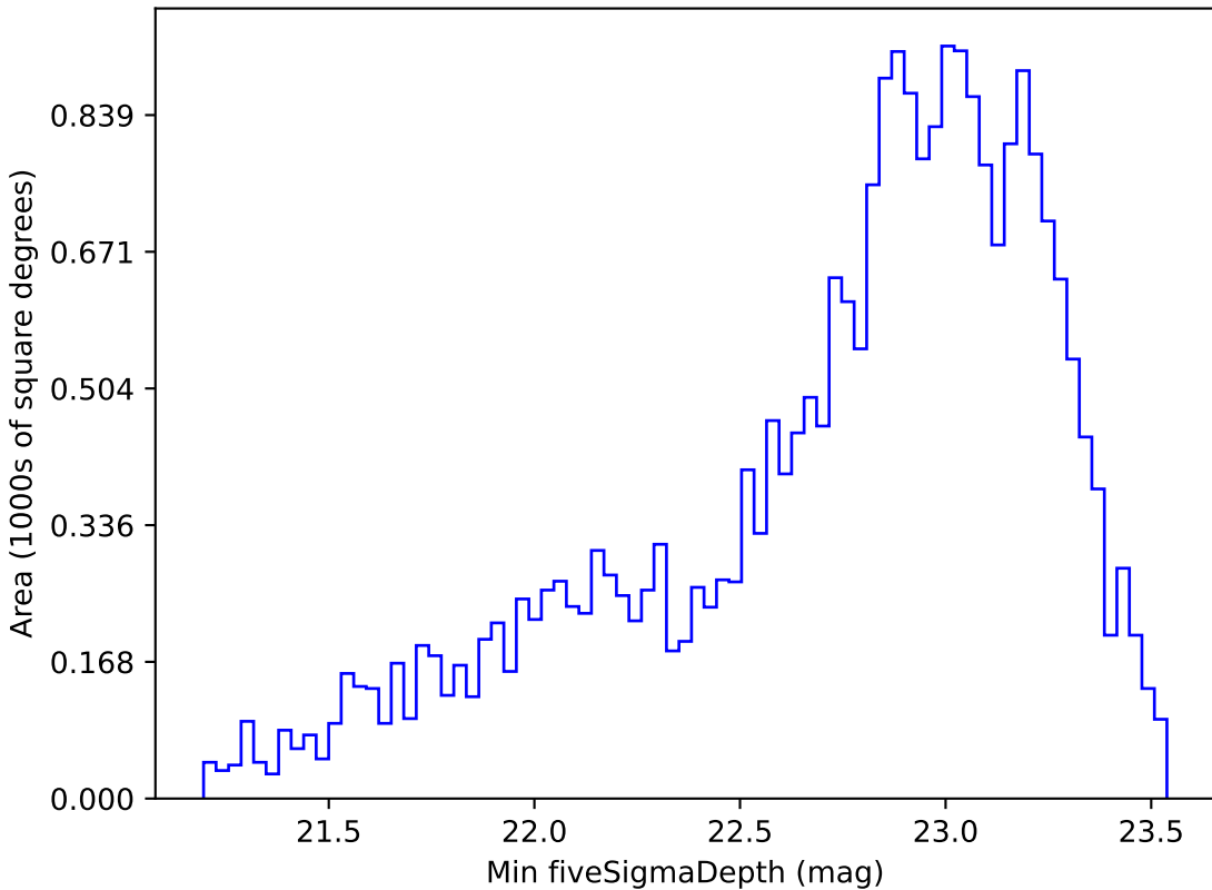
roman_v3.3_10yrs Yr 1 i band: Min fiveSigmaDepth
