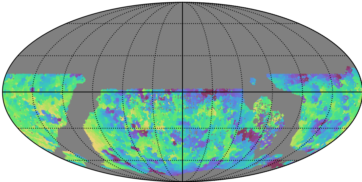
roman_v3.3_10yrs WFD u band: Min fiveSigmaDepth
