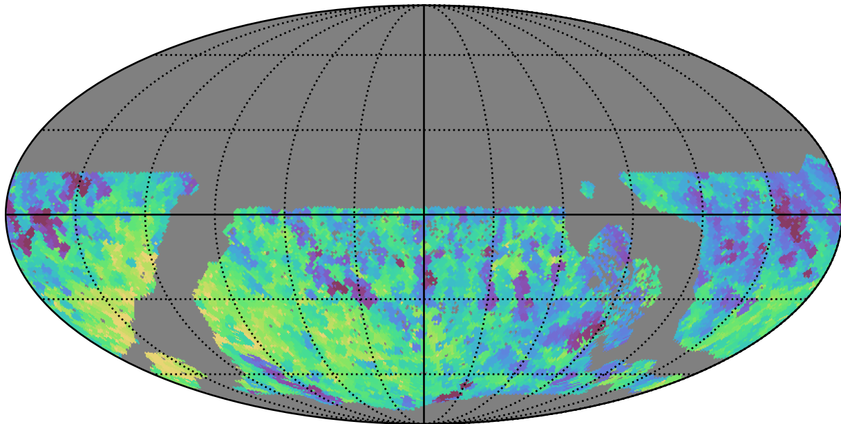
roman_v3.3_10yrs WFD all bands: Min fiveSigmaDepth
