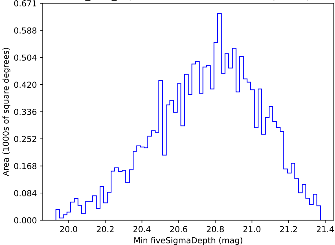
roman_v3.3_10yrs WFD all bands: Min fiveSigmaDepth
