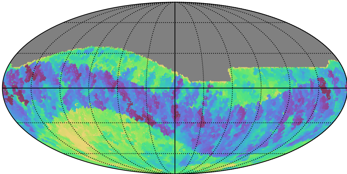
roman_v3.3_10yrs All sky z band: Min fiveSigmaDepth
