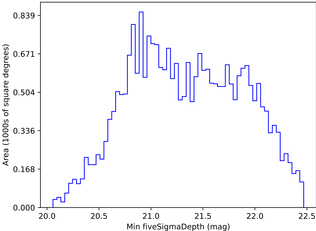
roman_v3.3_10yrs All sky z band: Min fiveSigmaDepth
