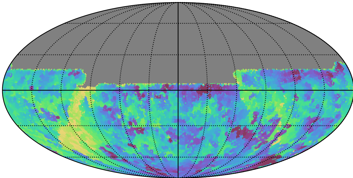
roman_v3.3_10yrs All sky u band: Min fiveSigmaDepth
