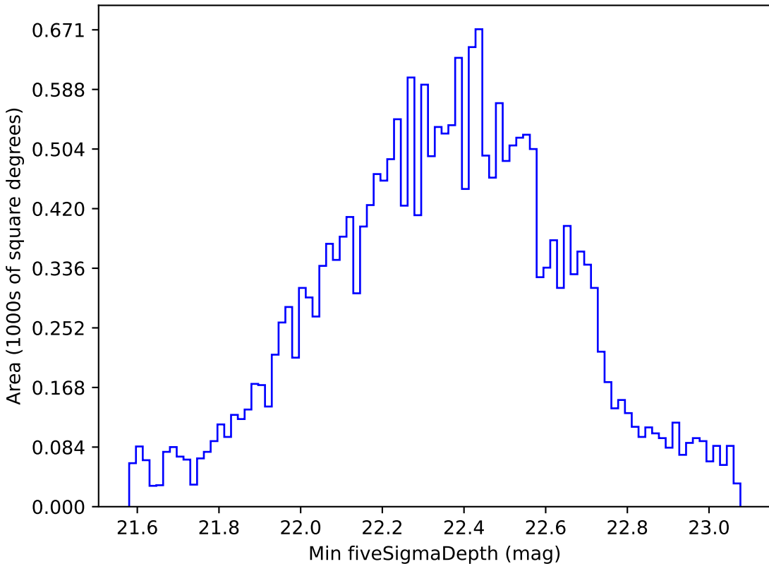
roman_v3.3_10yrs All sky u band: Min fiveSigmaDepth
