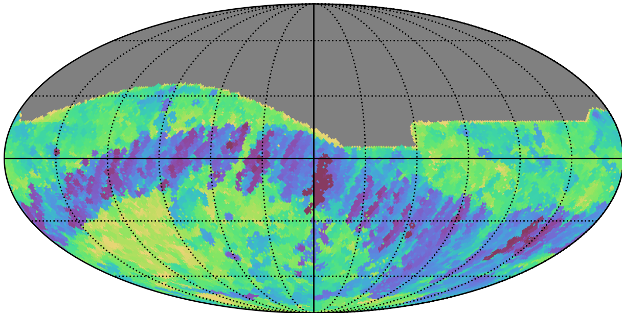
roman_v3.3_10yrs All sky r band: Min fiveSigmaDepth
