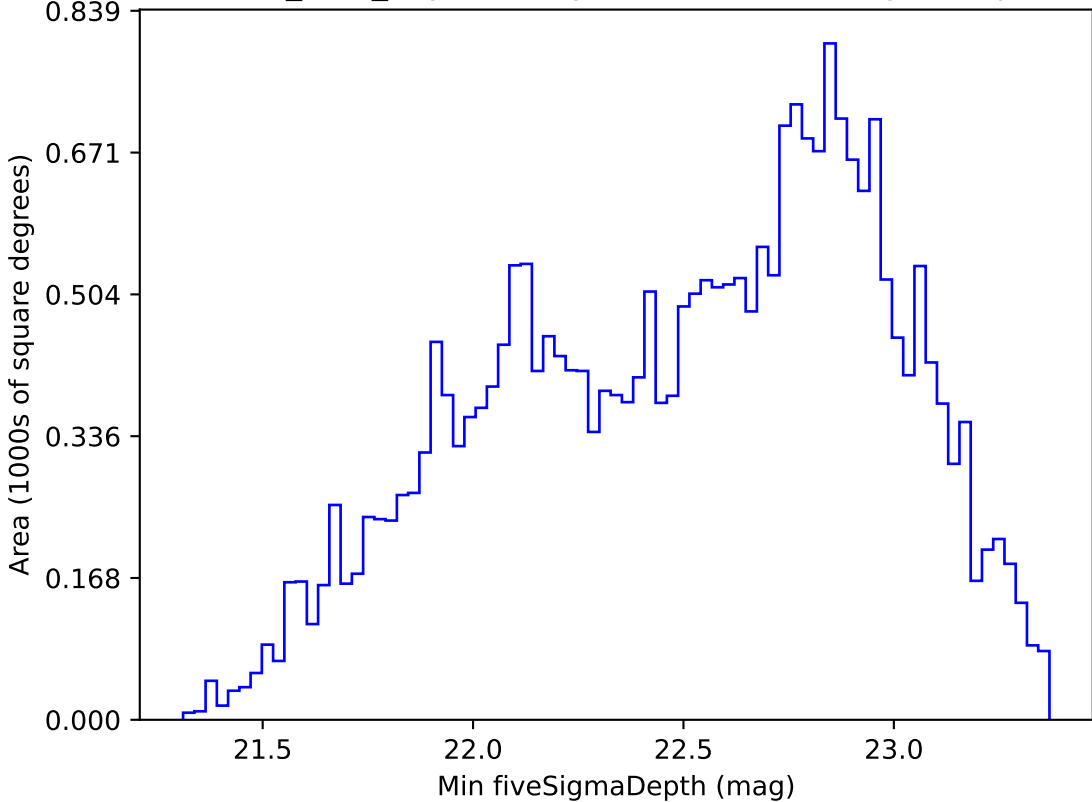
roman_v3.3_10yrs All sky r band: Min fiveSigmaDepth
