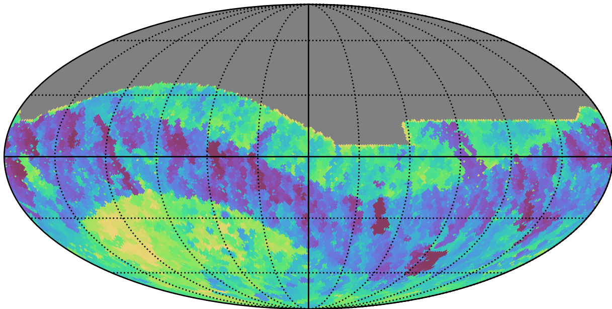
roman_v3.3_10yrs All sky i band: Min fiveSigmaDepth
