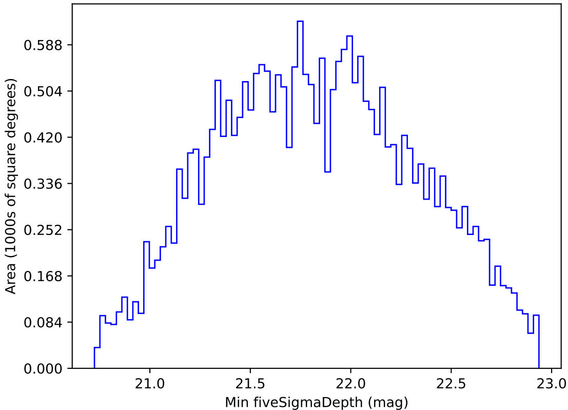
roman_v3.3_10yrs All sky i band: Min fiveSigmaDepth
