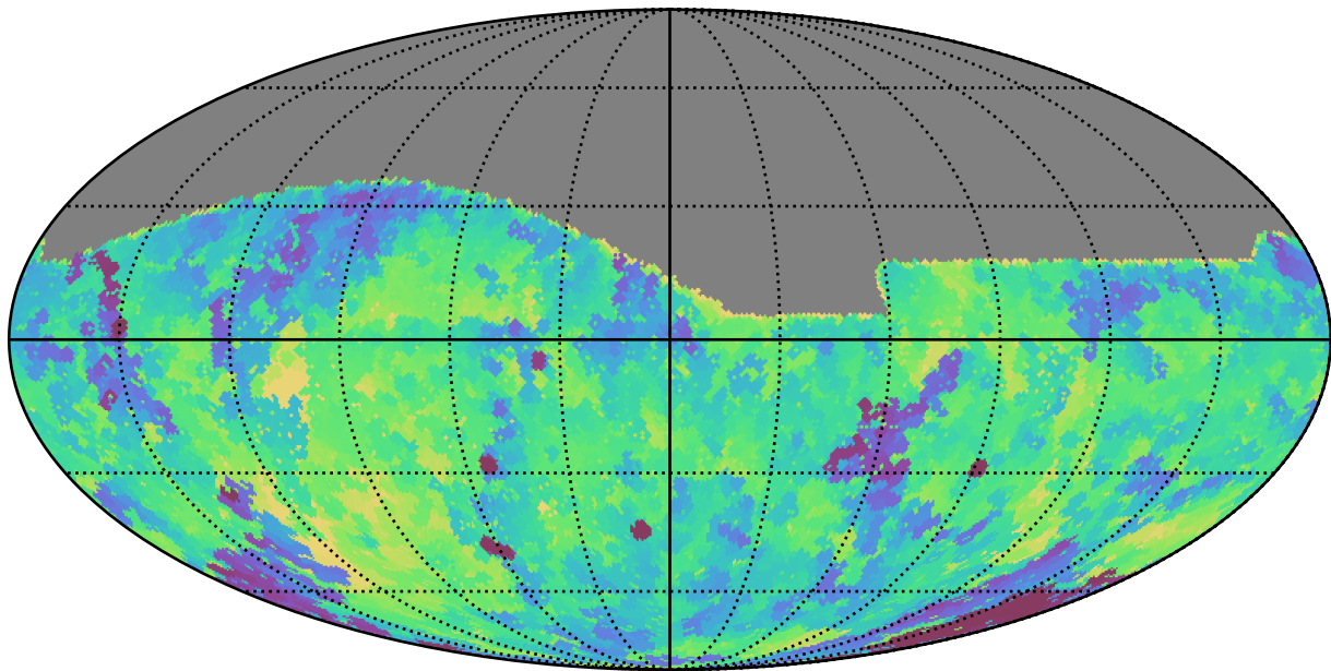
roman_v3.3_10yrs All sky g band: Min fiveSigmaDepth
