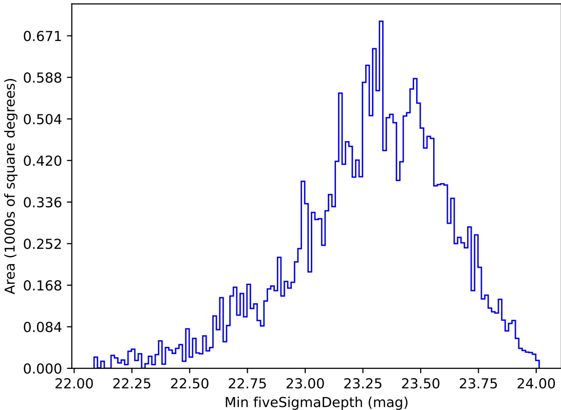
roman_v3.3_10yrs All sky g band: Min fiveSigmaDepth
