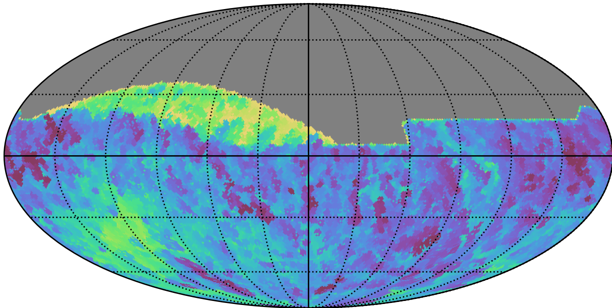
roman_v3.3_10yrs All sky all bands: Min fiveSigmaDepth
