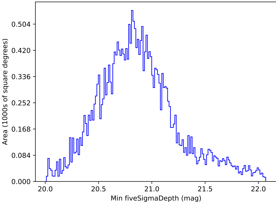
roman_v3.3_10yrs All sky all bands: Min fiveSigmaDepth
