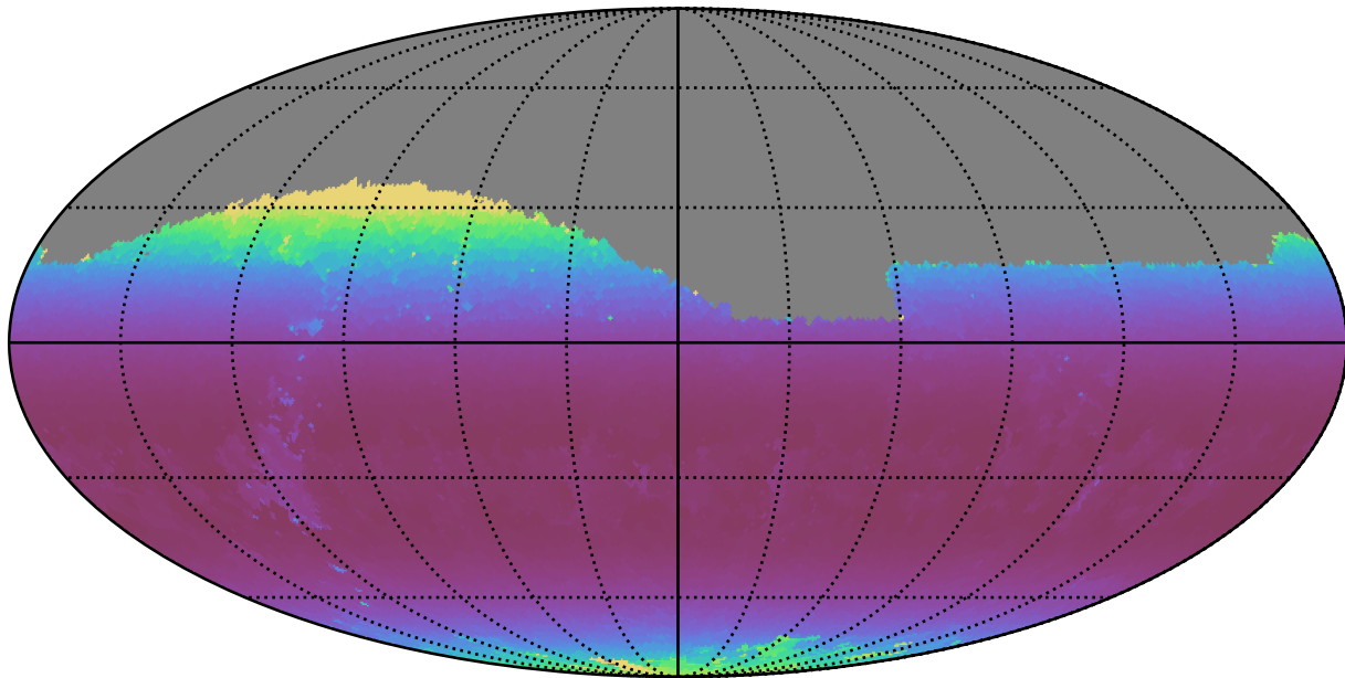
roman_v3.3_10yrs Yr 1 z band: Min airmass
